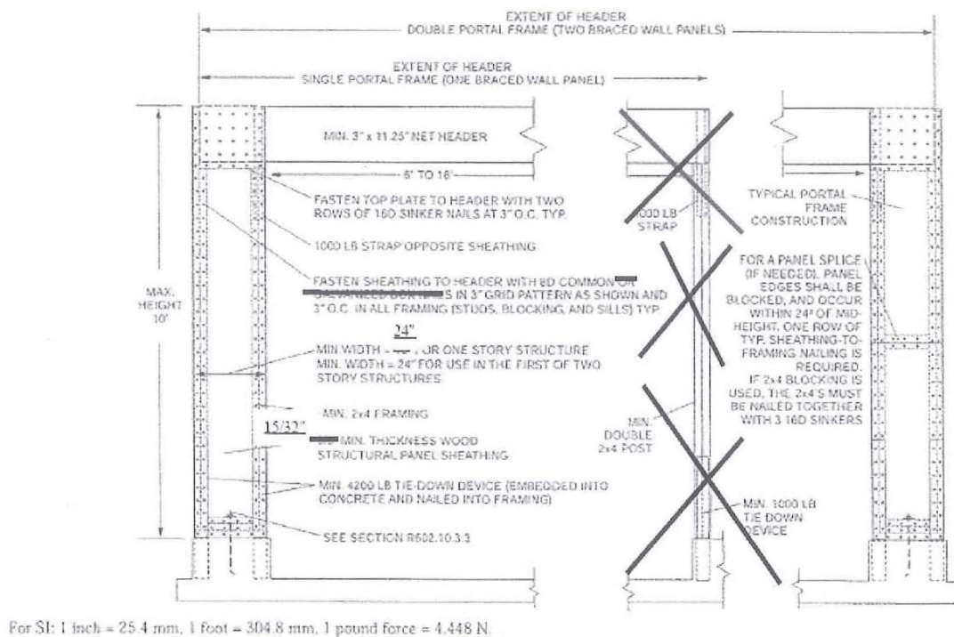
FIGURE R602.10.3.3 91.R602.10.3.3 METHOD PFH: PORTAL FRAME WITH HOLD-DOWNS
