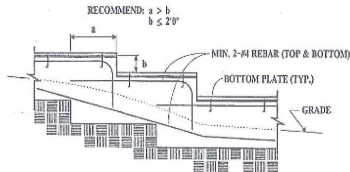
STEPPED FOUNDATIONS
