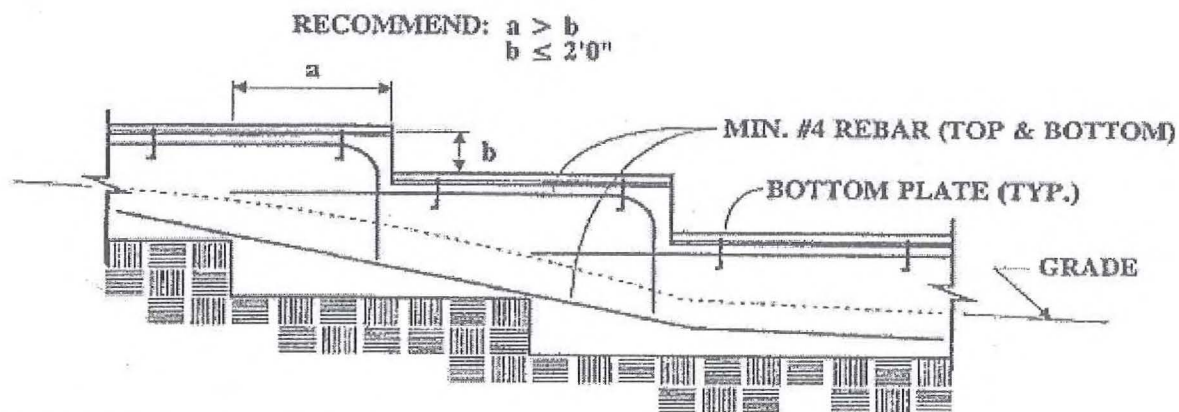
STEPPED FOUNDATIONS FIGURE 4805.4 1809.3
