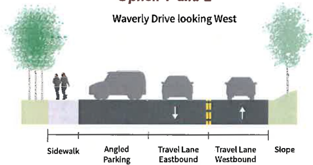
Figure 25 - Cross Section depicting Waverly Option 1 and 2
