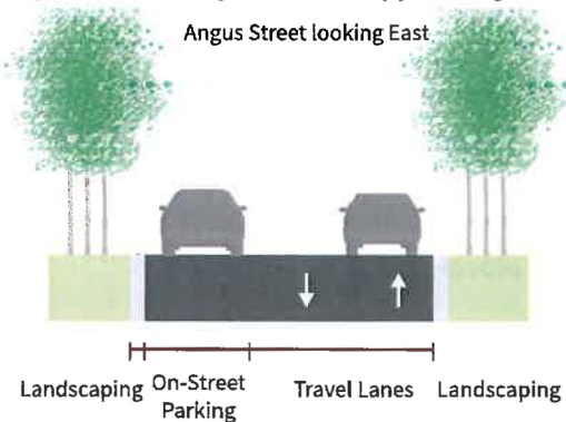
Figure 21 - Cross Section depicting Upper Angus Option 1
