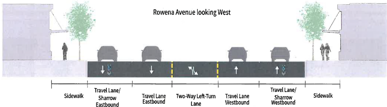
Figure 35 - Cross Section depicting Rowena Option 4
