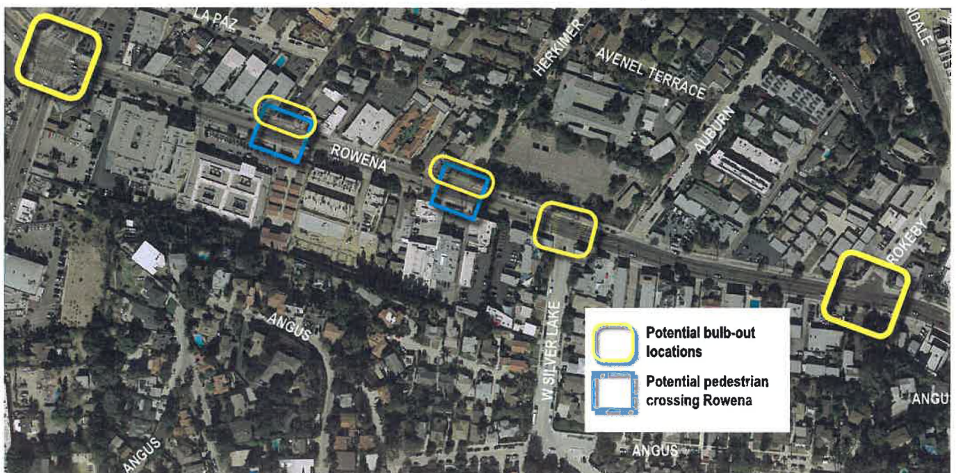
Figure 31 - Potential high-level locations of bulb-outs along Rowena Option 1a
