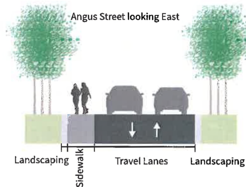
Figure 22 - Cross Section depicting Upper Angus Option 2
