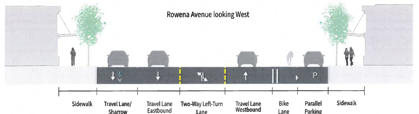
Figure 34 - Cross Section depicting Rowena Option 3
