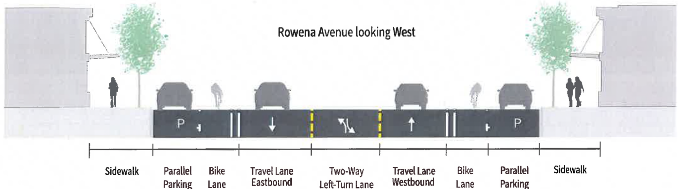
Figure 33 - Cross Section depicting Rowena Option 2
