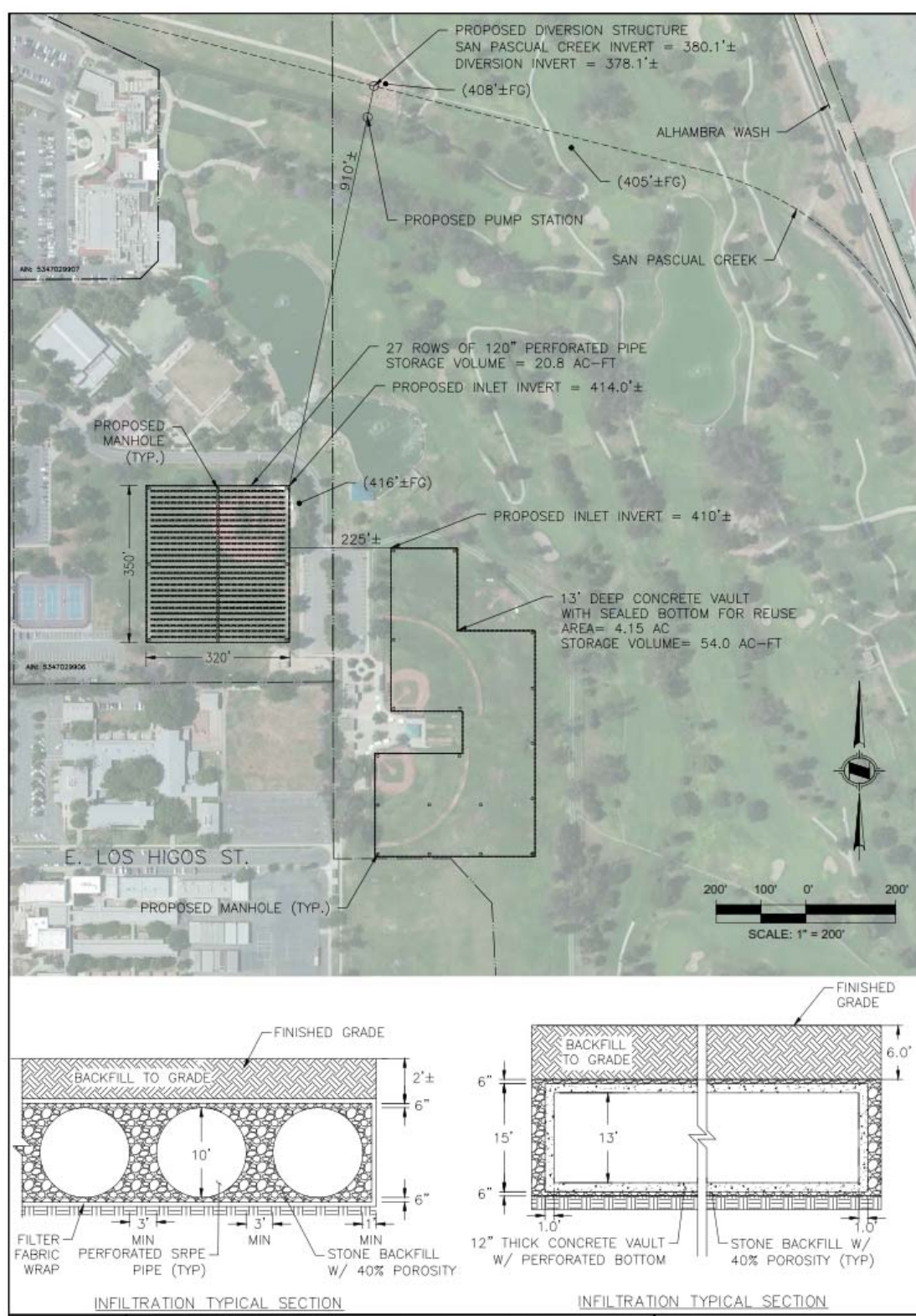
Figure 4-10. Alhambra Golf Course Preliminary Design
