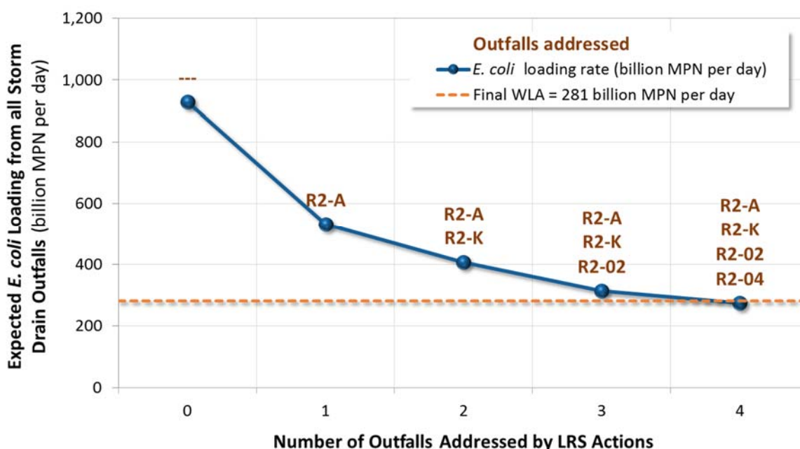
Figure 7-26. Effect of Priority Outfall Actions on E. coli Loading to Segment B from ULAR EWMP Group
