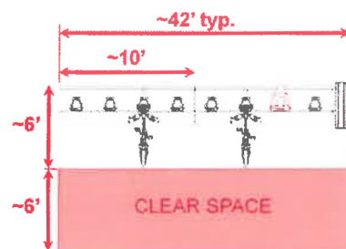
Figure 35 – Typical Modular Station Footprint
