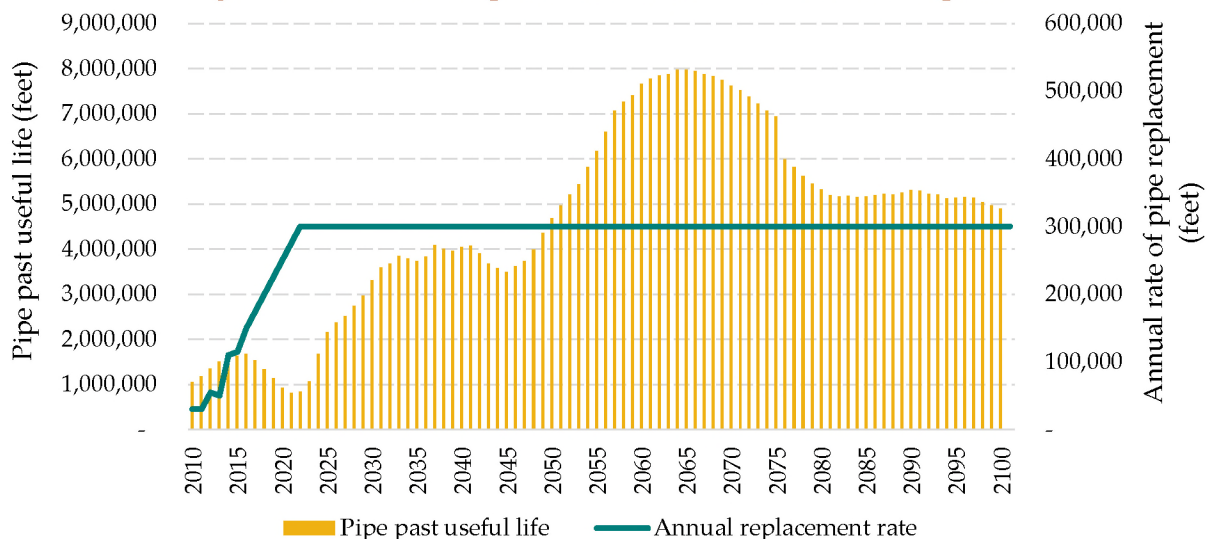
Figure 3-17. Mainline Replacement Based on Current Rate Proposal
