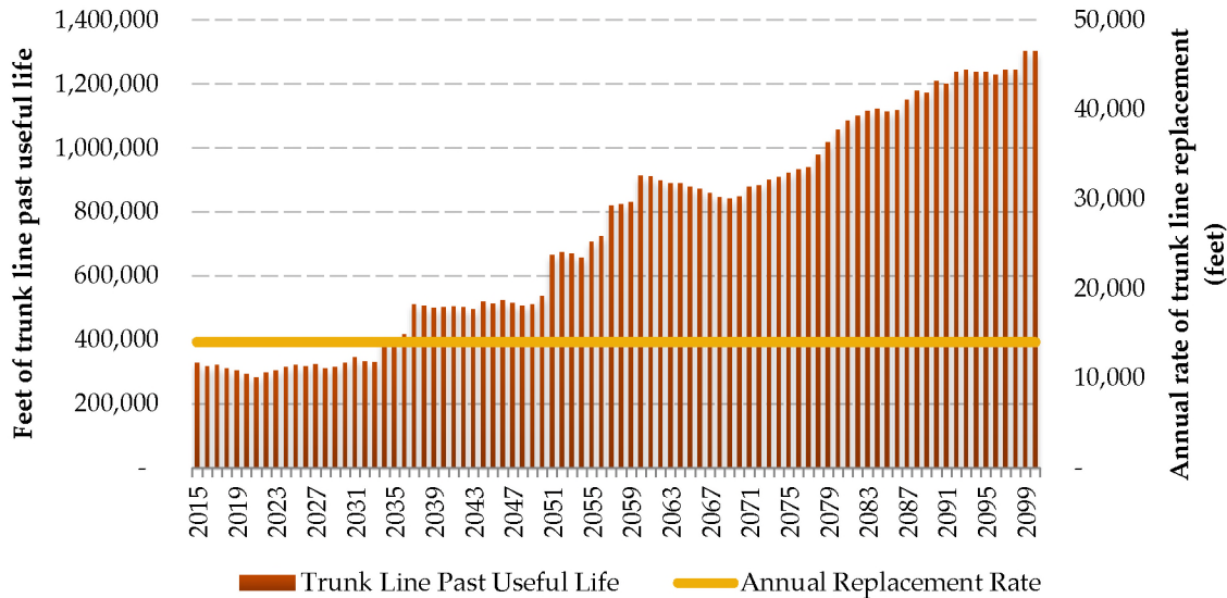
Figure 3-19. Trunk Line Replacement based on Historical Replacement Rate
