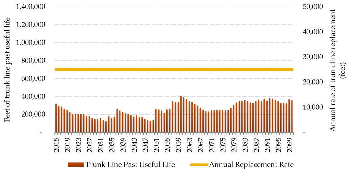
Figure 3-20. Trunk Line Replacement based on 25,000 feet/year Replacement Rate
