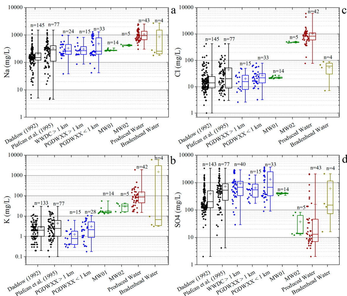
Figure 3. Box and whisker plots of minimum and maximum, quartiles, median (line in boxes), mean (crosses in boxes) of (a) Na, (b) K, (c) Cl, (d) SO 4 for domestic wells inventoried by Daddow 48,53 and Plafcan 51 in the Wind River Indian Reservation and Fremont County, respectively, sampled by EPA 6,8,9,39 and WDEQ 45 (PGDWXX series) greater than and less than 1 km from a production well, Wyoming Water Development Commission 52 (WWDC series) greater than 1 km from a production well, EPA monitoring wells 9,39 (Tables SI E2b, SI E3b), and produced water and bradenhead water samples (Table SI D1). Domestic wells sampled more than once, including data from Daddow 53 are represented with a mean value. Fourteen measurements in Daddow 53 < 1 mg/L for potassium are not illustrated. Data points at MW01 and MW02 are samples collected during Phase III, IV, and V sample events.
