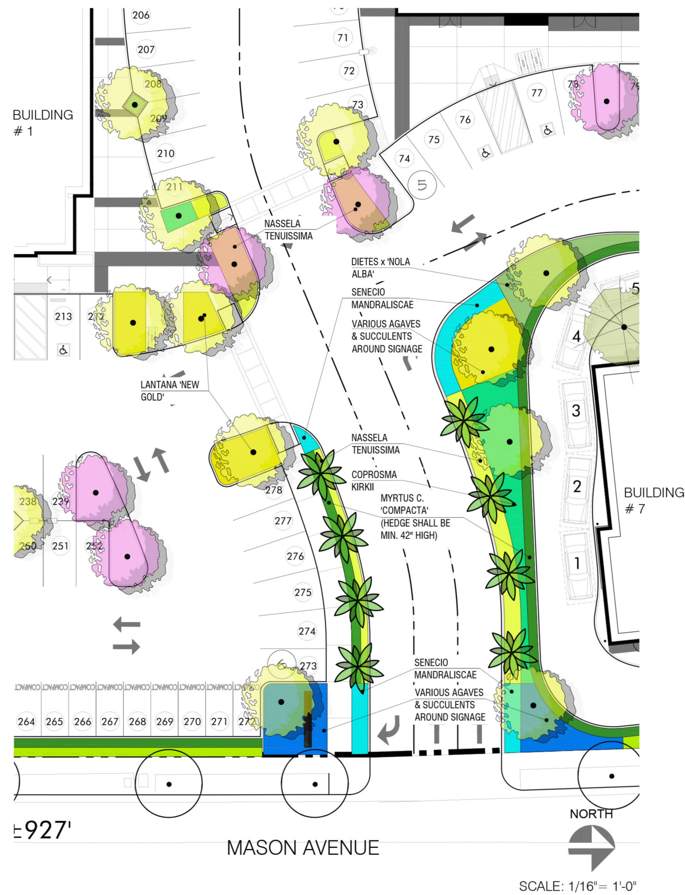
ENLARGEMENT PLAN: Vehicular Entrance from Mason Avenue A
