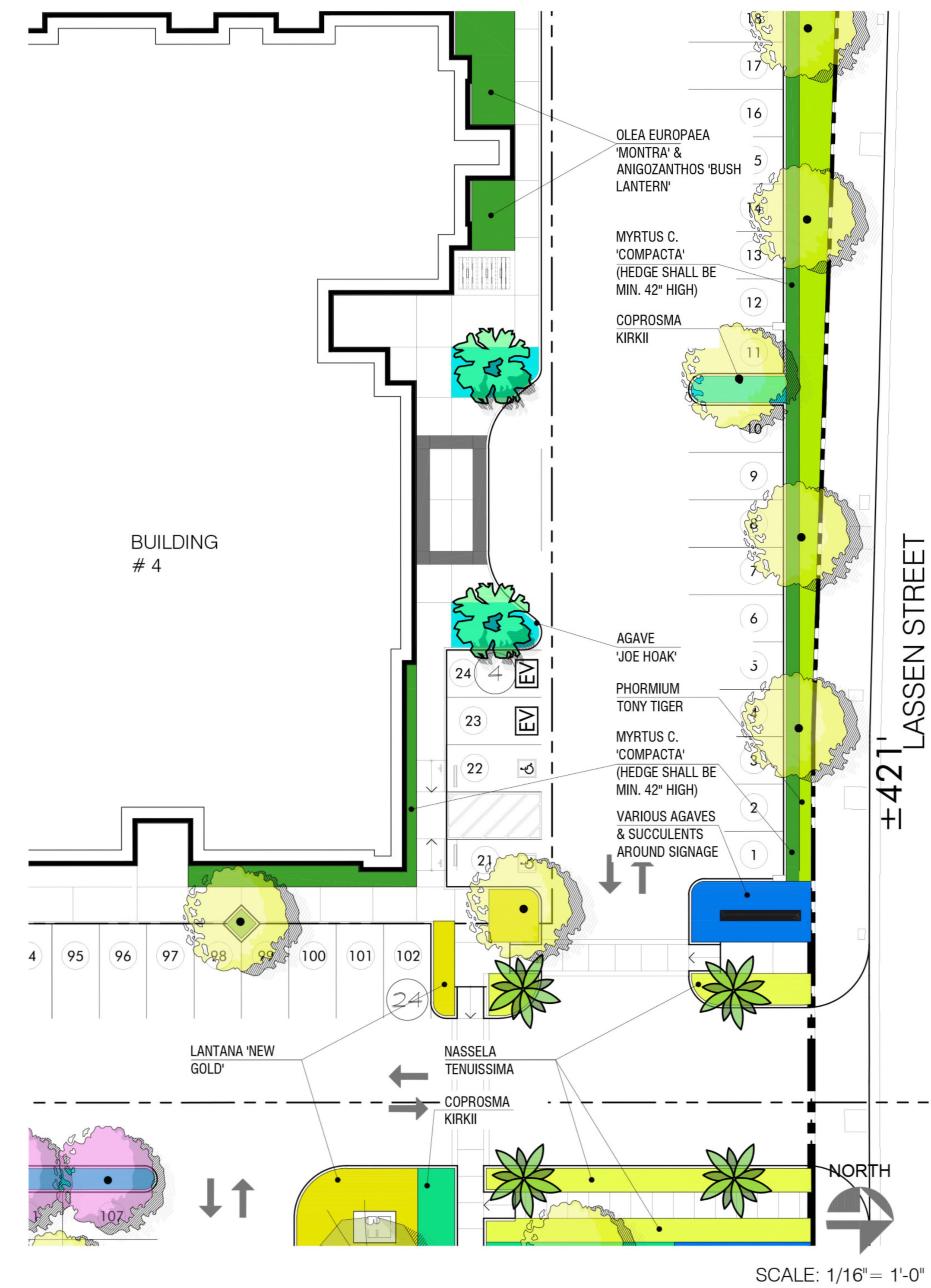
ENLARGEMENT PLAN: Vehicular Entrance from Lassen Street C
