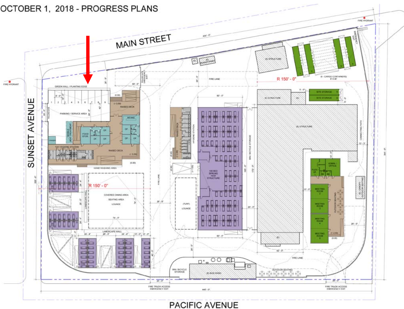
Project Site Plan (from 11/29/18 Department of Public Works Report)
