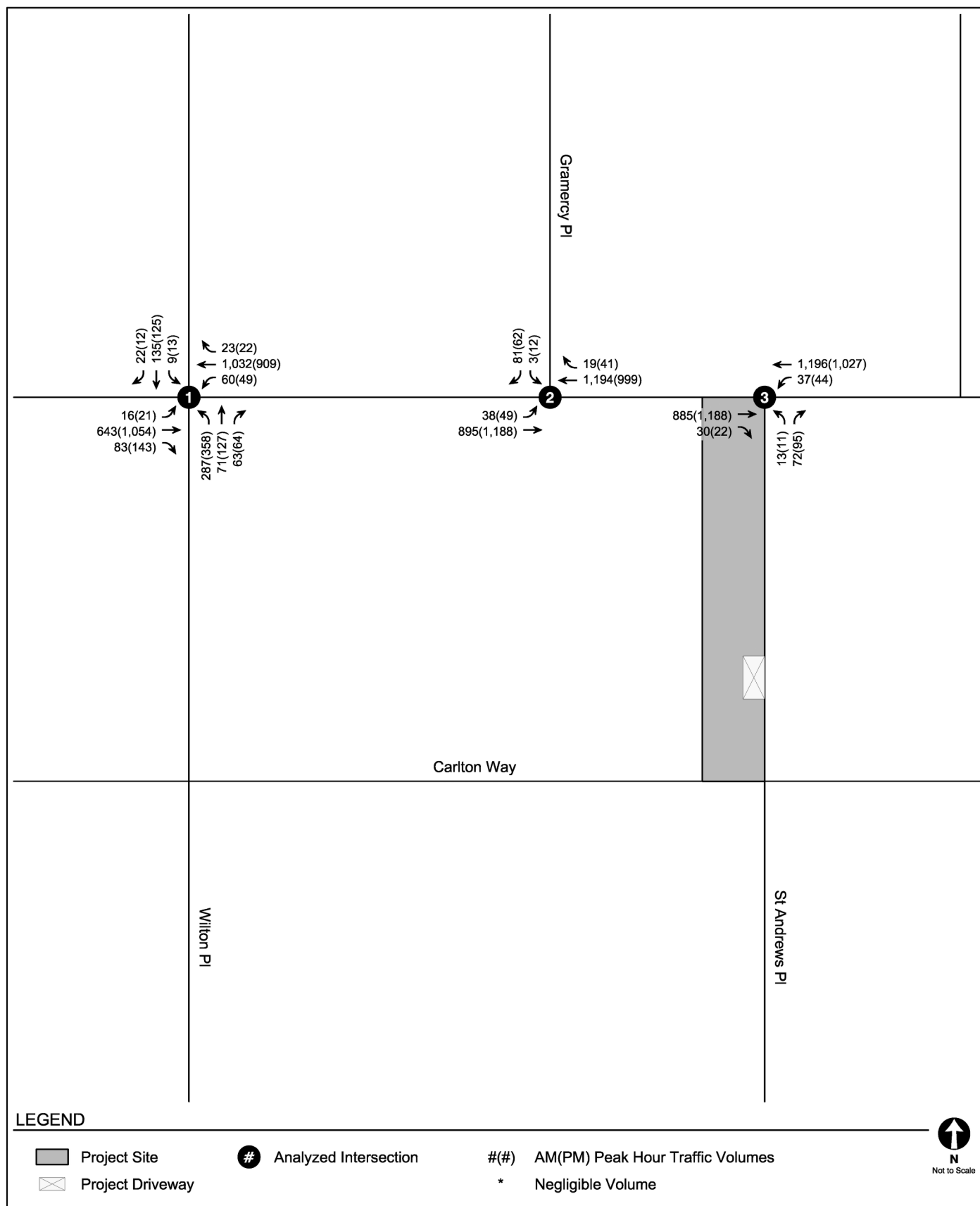
EXISTING CONDITIONS (YEAR 2020) PEAK HOUR TRAFFIC VOLUMES
