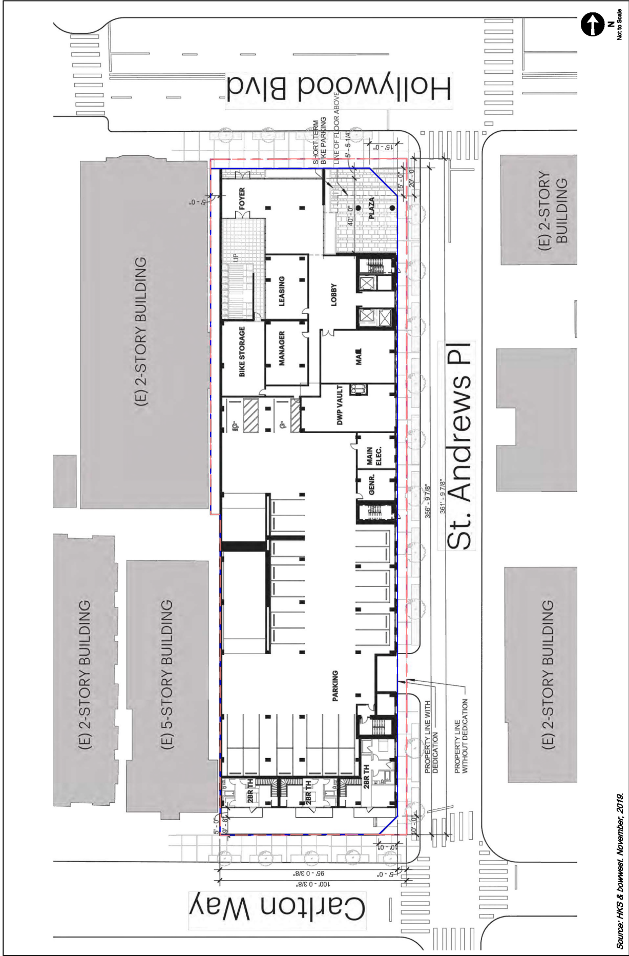
PROJECT SITE PLAN
