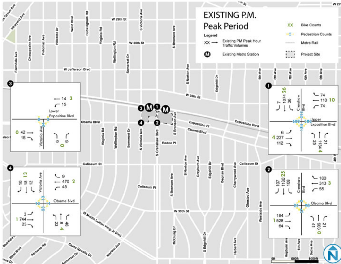
Figure 5-2 Existing Study Intersection Vehicle Turning Movement Volumes (PM Peak Hour)
