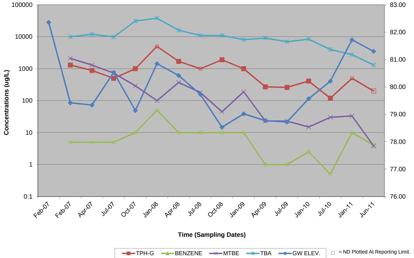
Graph 3 - TPH-g, Benzene, MTBE, TBA Concentrations vs. Time (MW-5)
