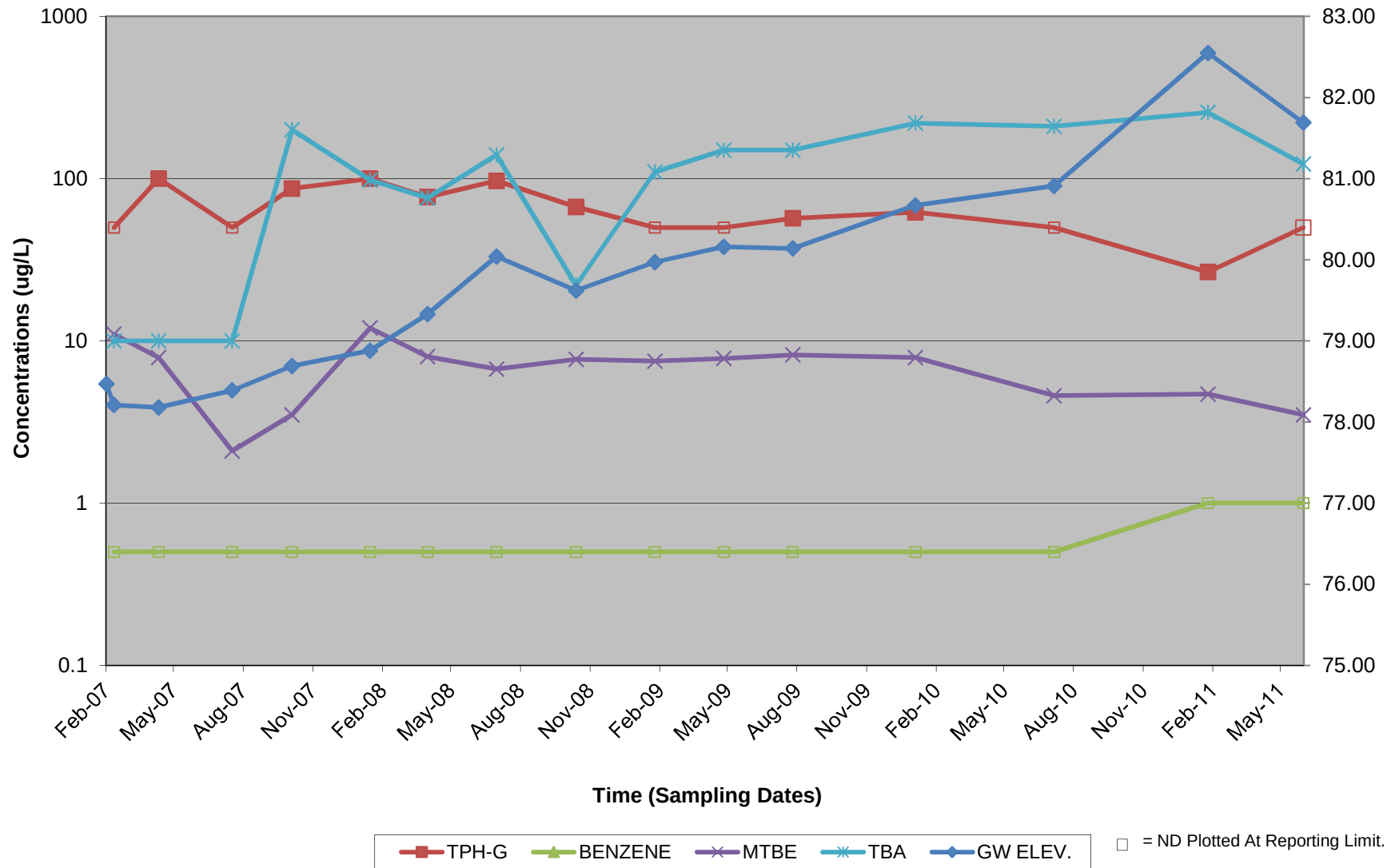
Graph 1 - TPH-g, Benzene, MTBE, TBA Concentrations vs. Time (MW-2)
