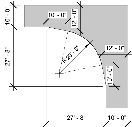
TURNING RADIUS - ONE WAY
