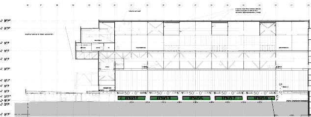
Overall Building Section Through Pico Looking South
