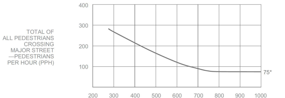
SPEED > 35 MPH Figure 4C-6. Warrant 4, Pedestrian Four-Hour Volume (70% Factor)
