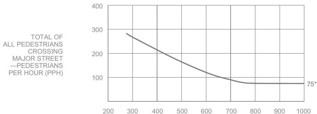
SPEED > 35 MPH Figure 4C-6. Warrant 4, Pedestrian Four-Hour Volume (70% Factor)
