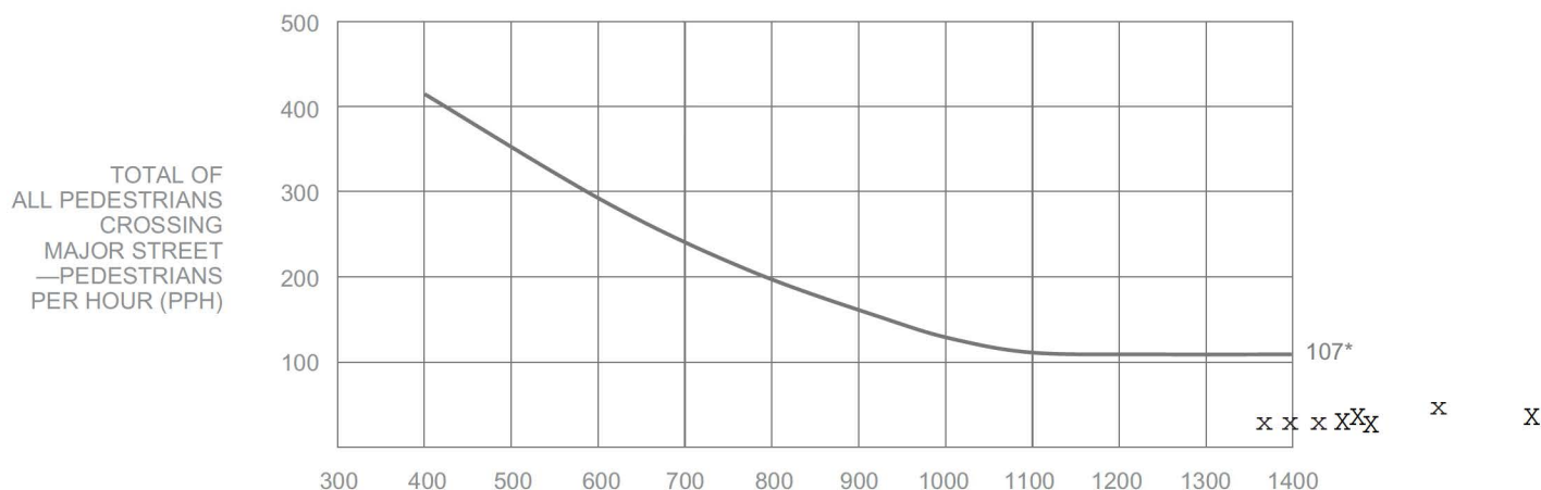
SPEED ≤ 35 MPH Figure 4C-5. Warrant 4, Pedestrian Four-Hour Volume
