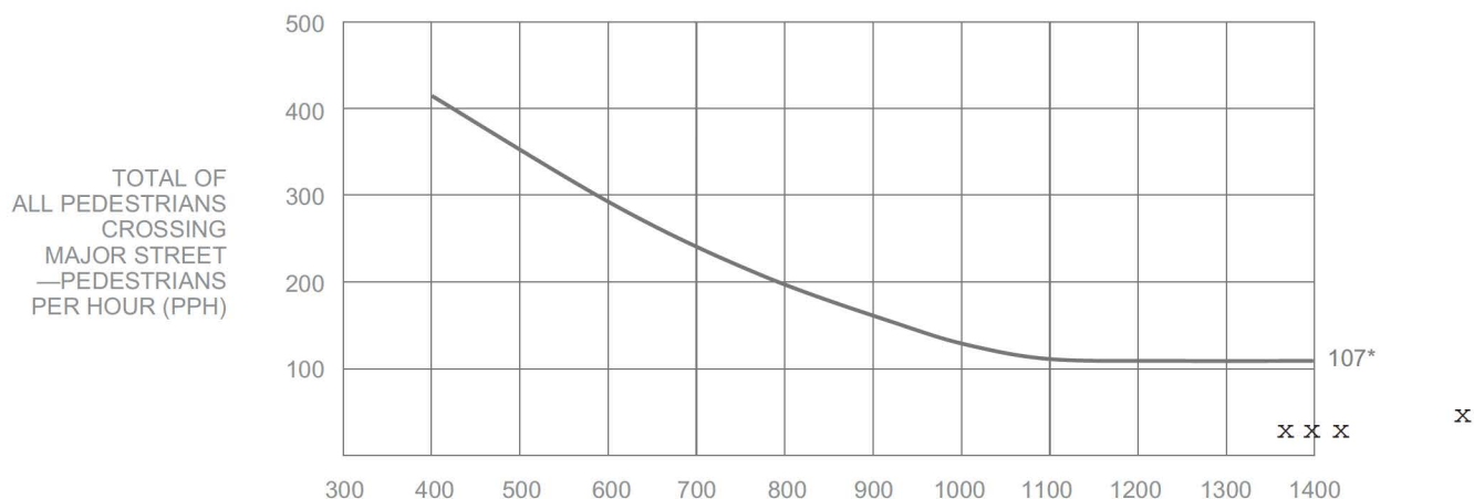
SPEED ≤ 35 MPH Figure 4C-5. Warrant 4, Pedestrian Four-Hour Volume
