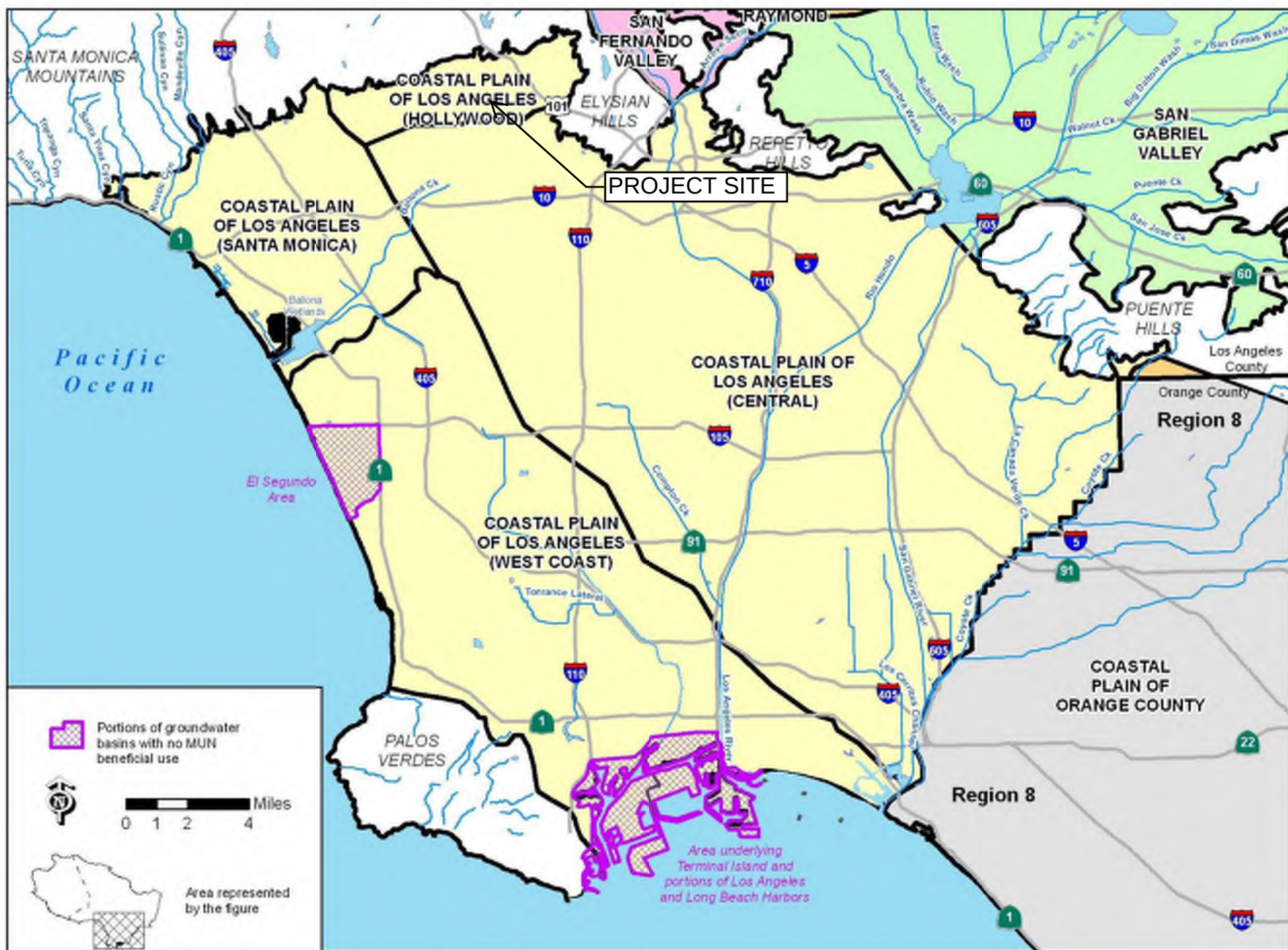
Figure 3: Coastal Plain of Los Angeles Groundwater Basin
