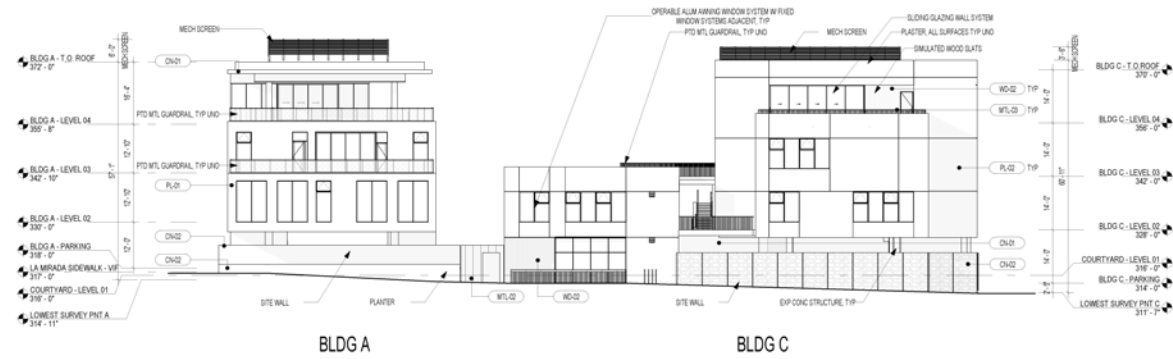
OVERALL WEST ELEVATION 1/8" = 1'-0" 3
