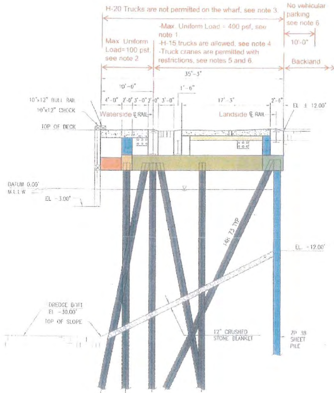
Wharf Restrictions and Allowances Sketch.
