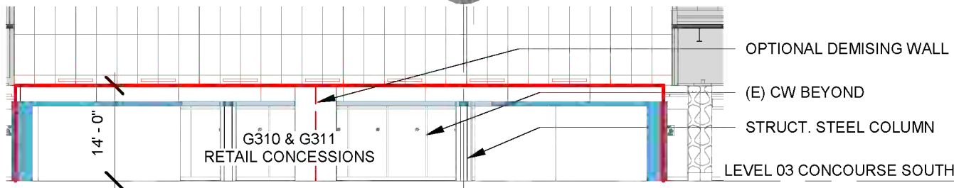
ELEVATION - G310 & G311 RETAIL CONCESSION ALT. - 2/A.114B
