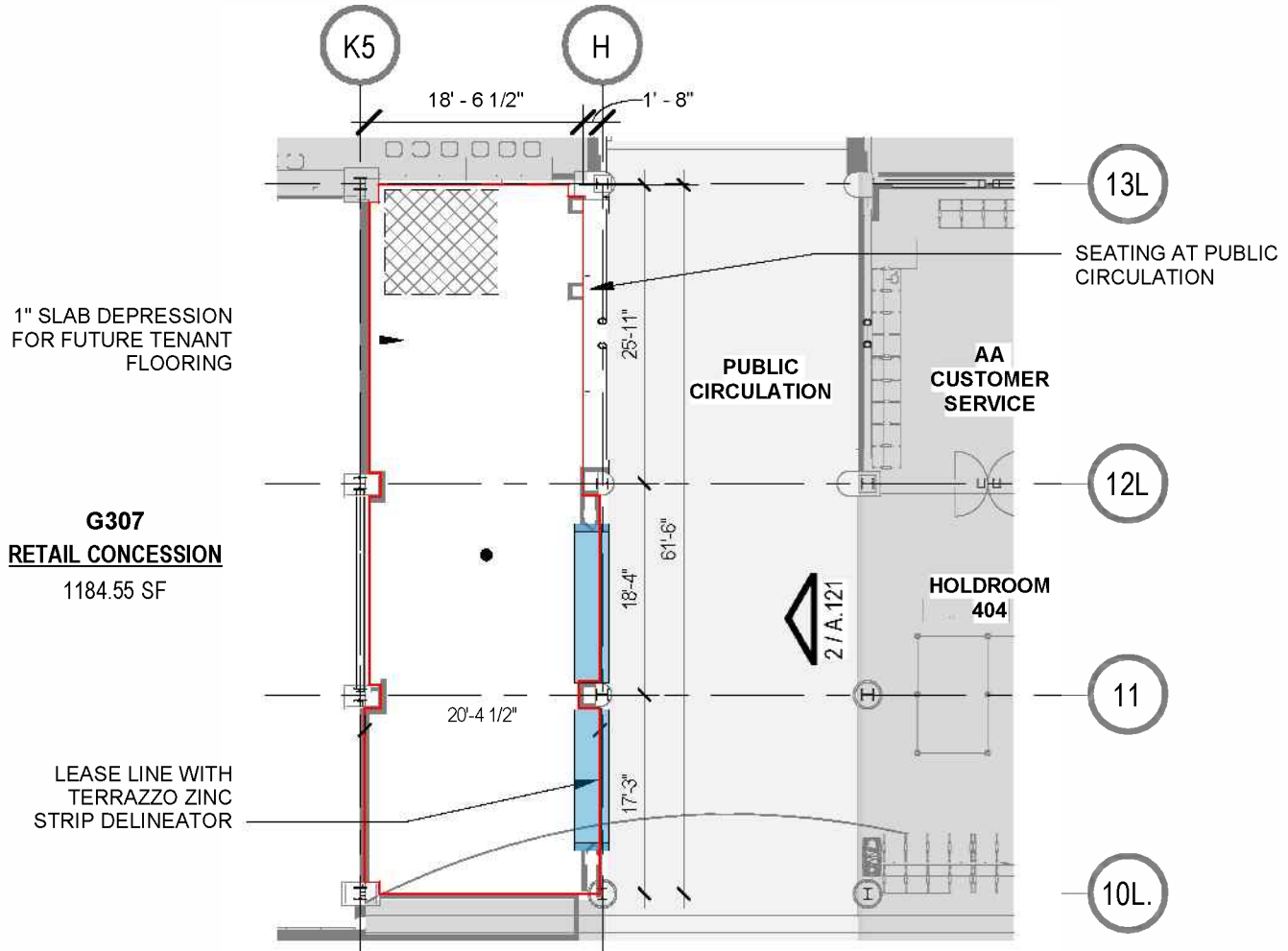
FLOOR PLAN - CONCOURSE LEVEL 03 - G307 RETAIL CONCESSION
