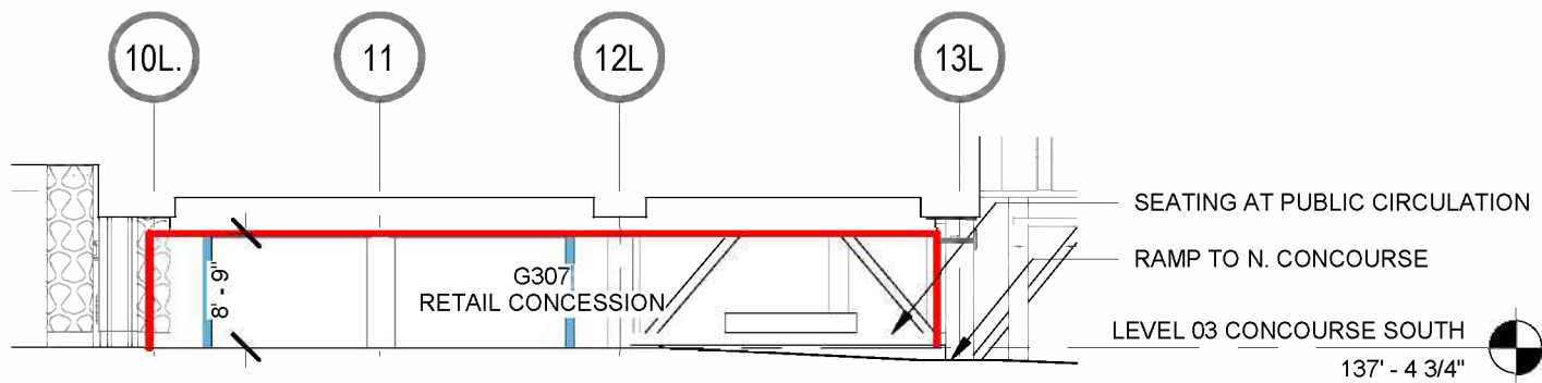
ELEVATION - G307 RETAIL CONCESSION - 2/A.121
