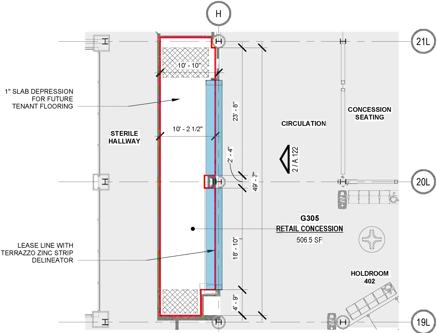
FLOOR PLAN - CONCOURSE LEVEL 03 - G305 RETAIL CONCESSION
