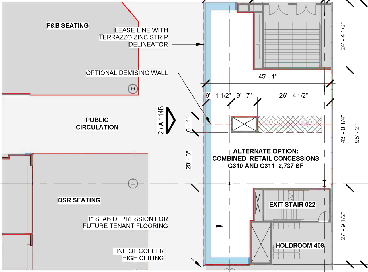
FLOOR PLAN - CONCOURSE LEVEL 03 - G310 & G311 RETAIL CONCESSION ALT.
